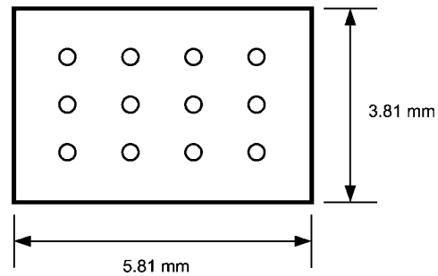
Exposed thermal pad mounting area.
